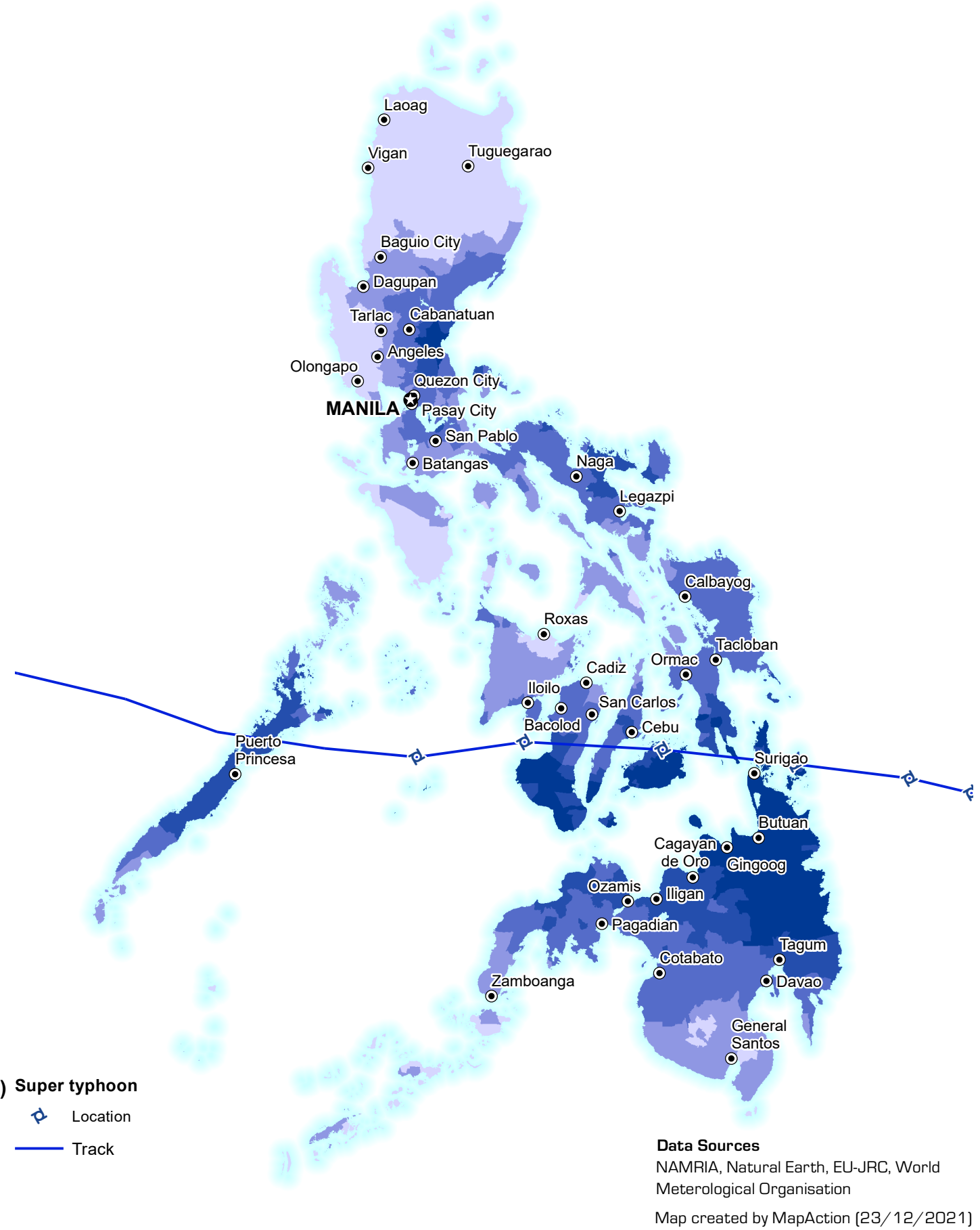
7 day cumulative rainfall in mm (13th - 19th December)
