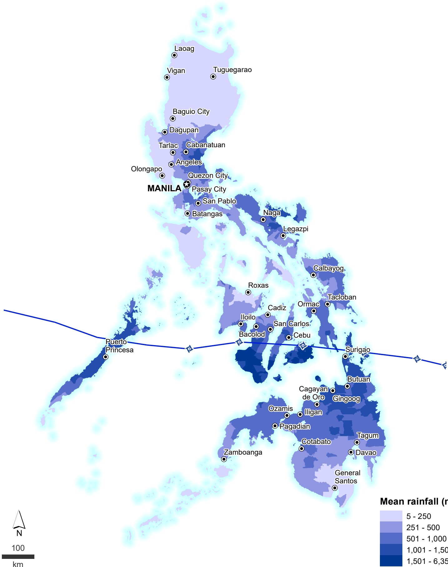
3 day cumulative rainfall in mm (16th - 18th December)
